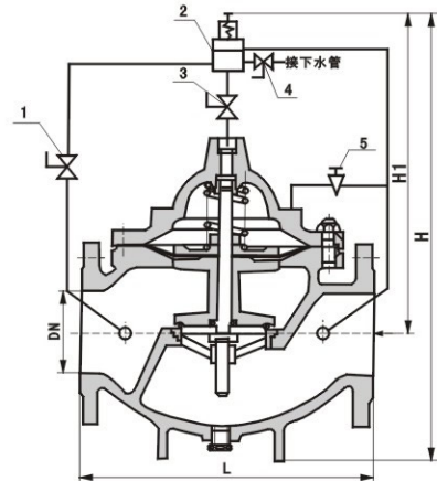
1 little ball valve 2 pilot valve 3 little ball valve 4 little valve 5 needle valve
