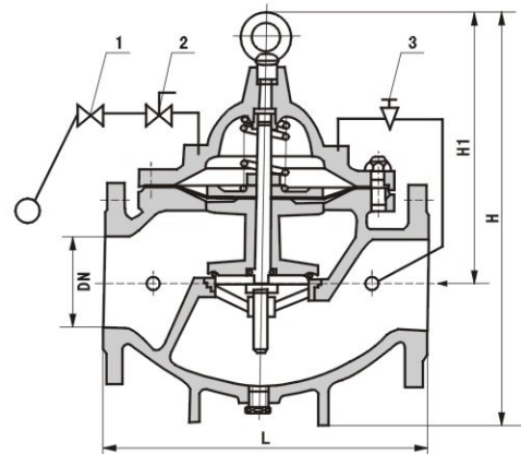
1, float pilot valve 2 ball valve 3 needle valve
